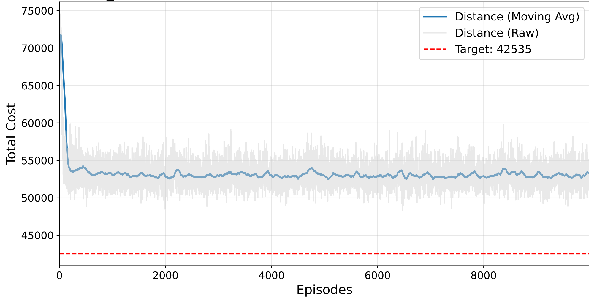
Final NO_BAYESIAN Masked AutoRL-SOP (HyperTuningSK) Training - ft70.3.sop
